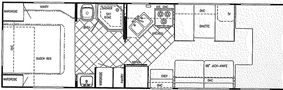
Model W6301D (Sofa Opt, Barrel Chairs Opt, Twin Beds or Bunks Opt.)
