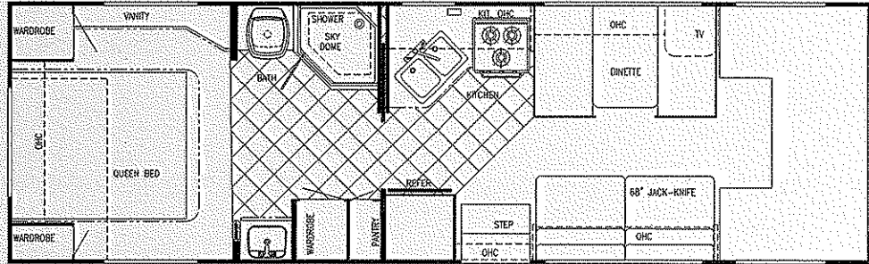
MODEL W6301Q (Sofa Opt, Barrel Chairs Opt, Twin Beds Opt.)
