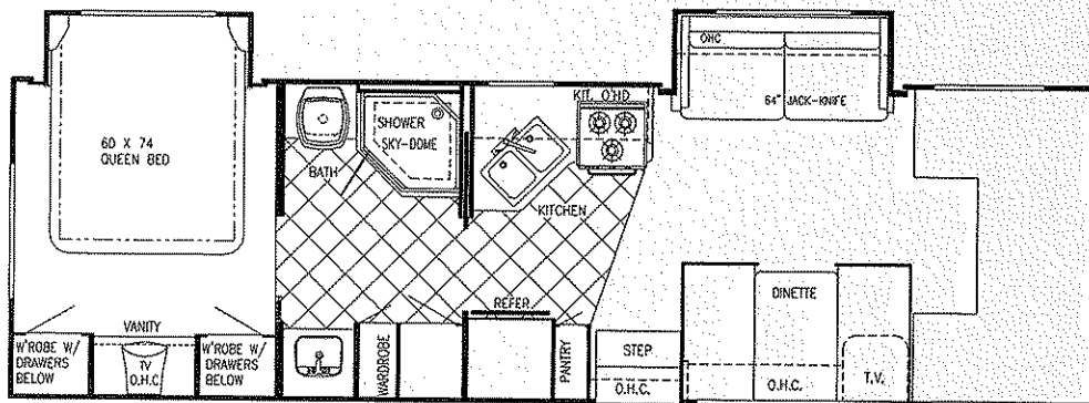
Model W6302D (Sofa, Barrel Chairs, or Free-Standing Dinette Opt)
