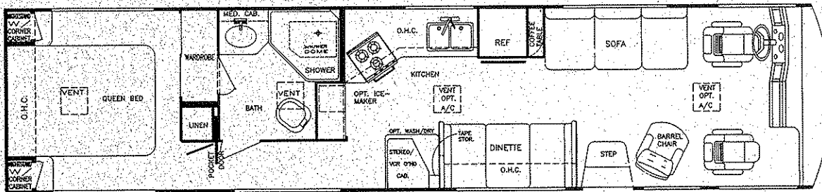
Model 8391 (Side Door Entry)
