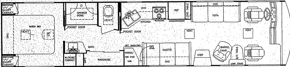
Model 8390 (Side Door Entry)
