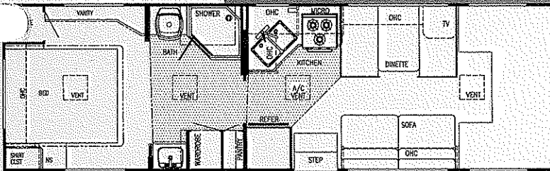
Model 6301 Wide-Body (Twin Beds or Bunks Opt.)
