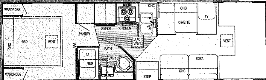
Model F6293HR (Twin Beds or Bunks Opt.)
