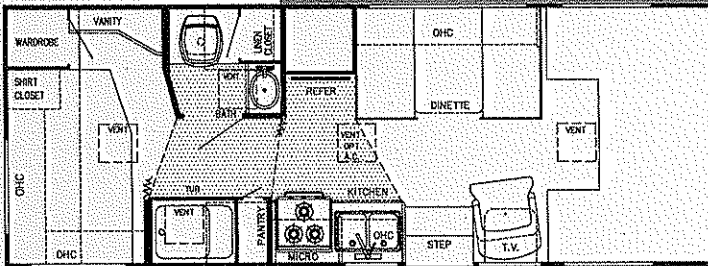
Model W6242 (Wide Body)
